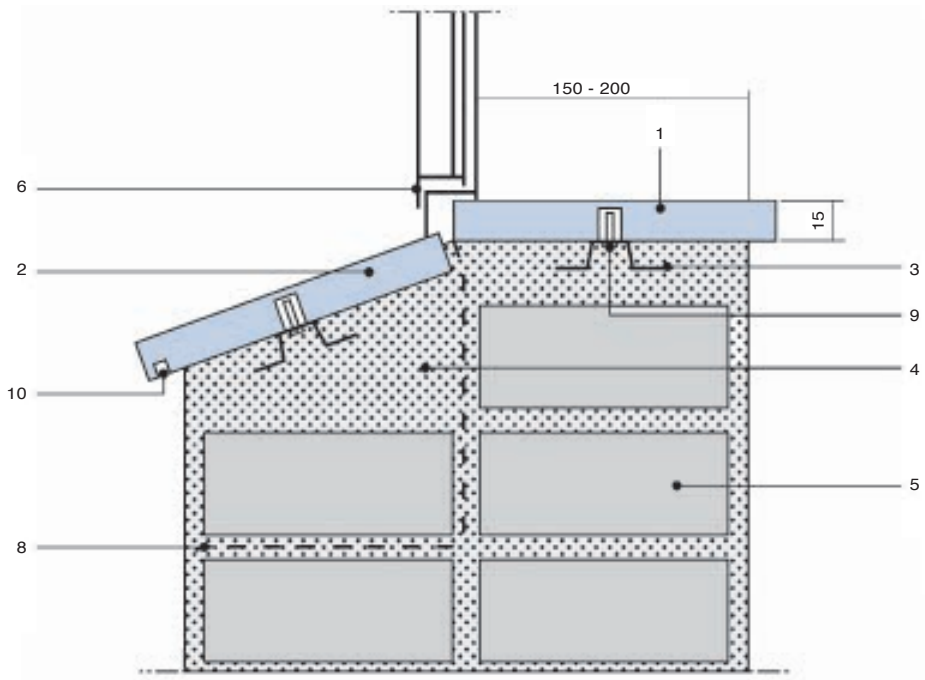
Fig 1 : Section showing internal and external sills in position
